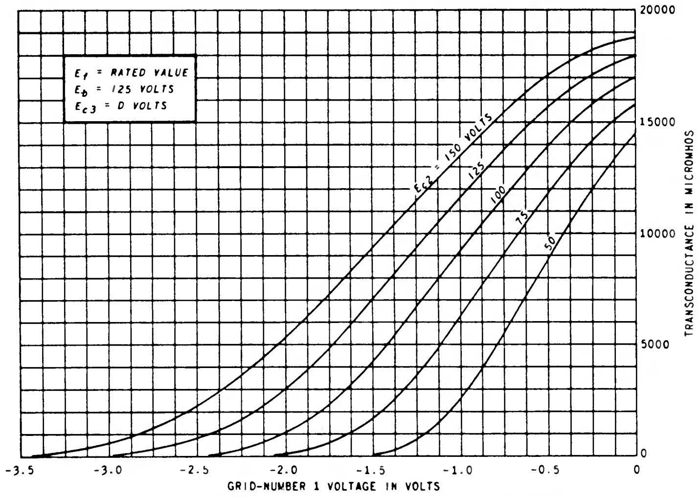
FIGURE 6, 6BN11 AVERAGE TRANSFER CHARACTERISTICS
