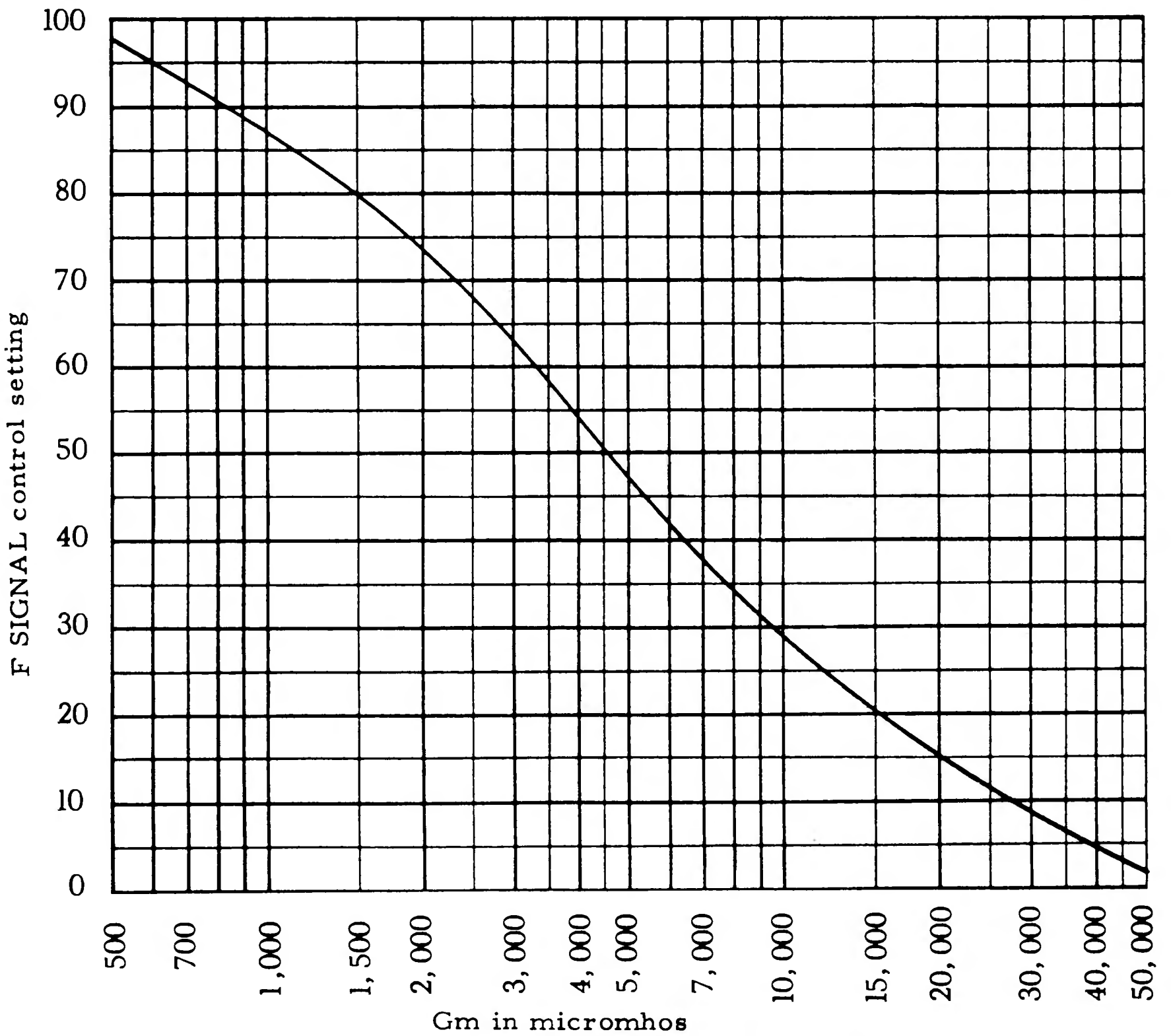
FIGURE 7, MU140 CONVERSION CHART
